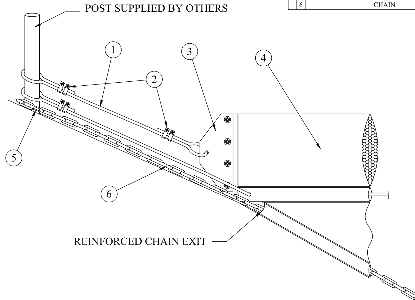
BAFFLE-ANCHOR CONNECTION
